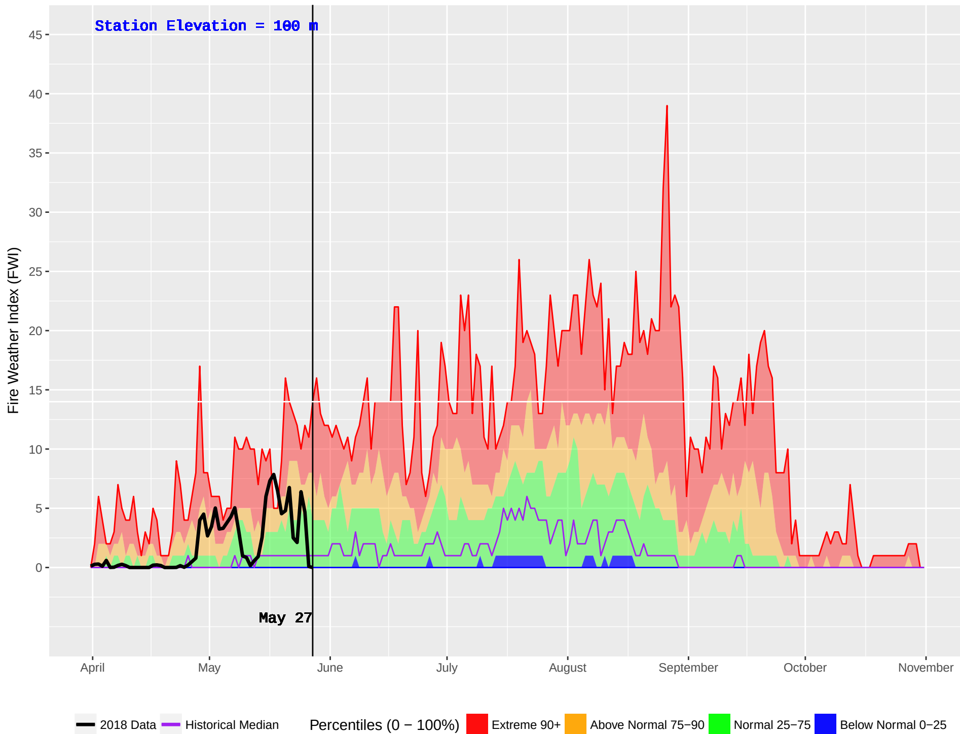
HONNA (93) : Historical (1986–2016) and Current (2018) Noon Fire Weather Index (FWI)
