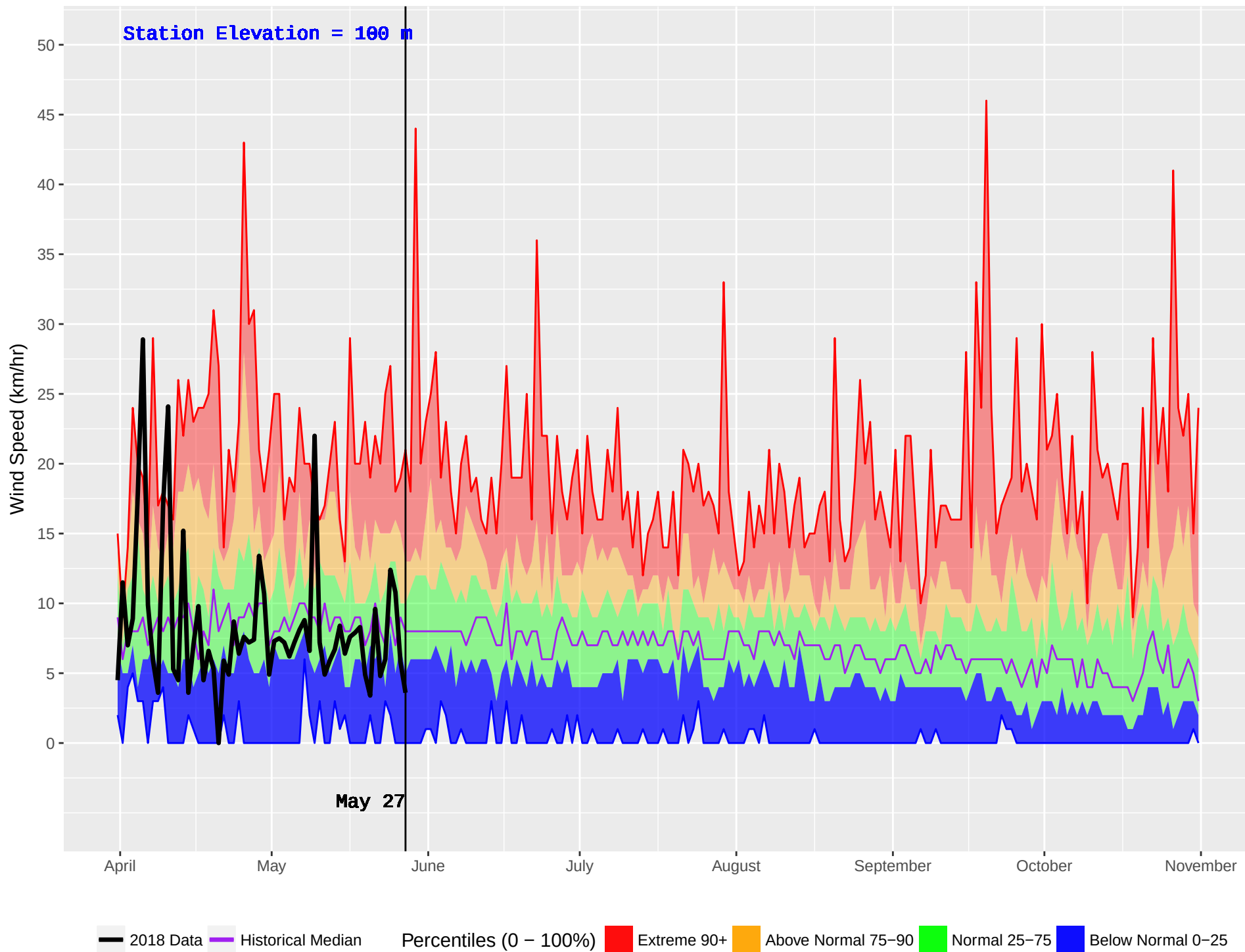
HONNA (93) : Historical (1986–2016) and Current (2018) Noon Wind Speed
