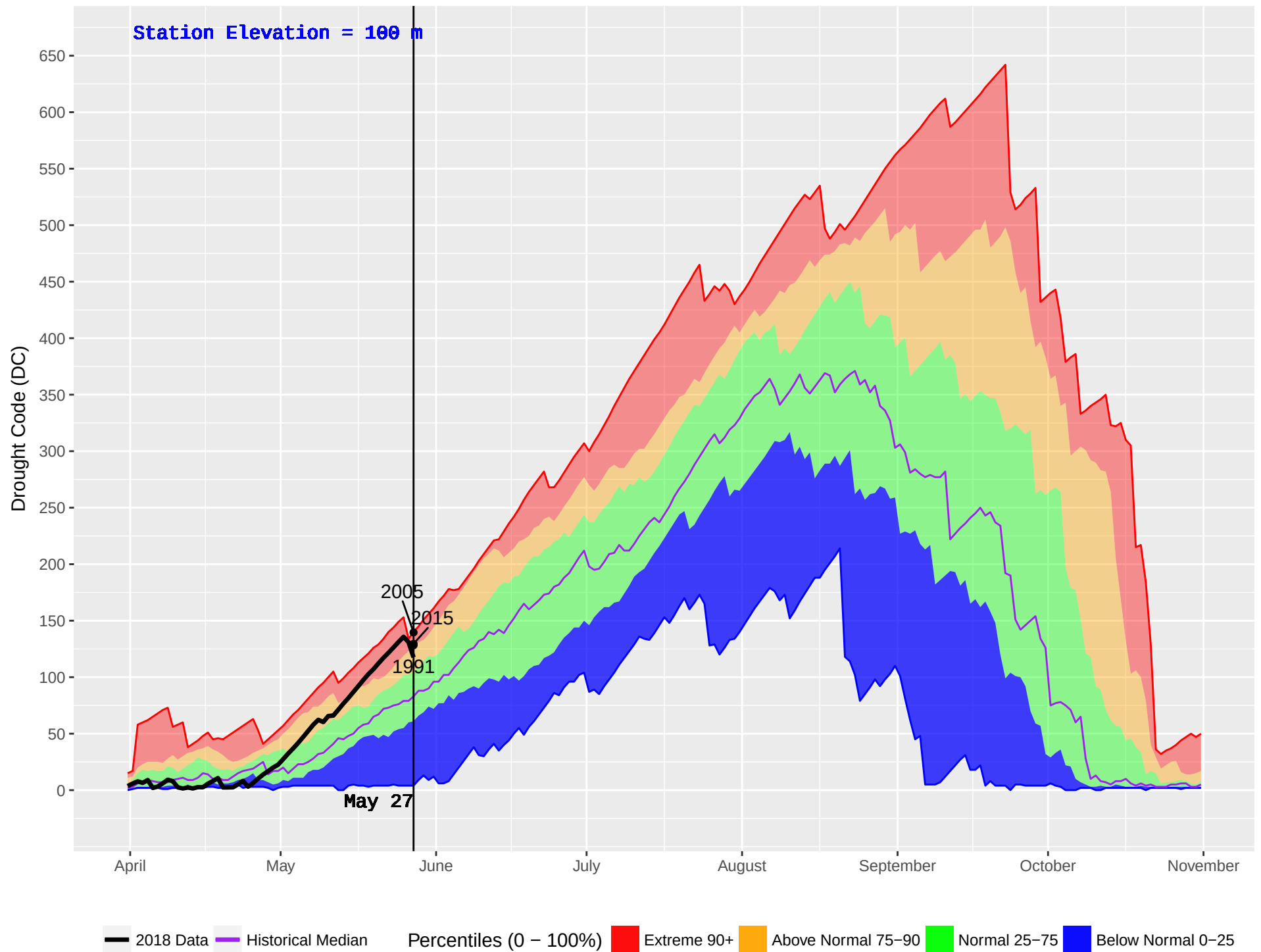
HONNA (93) : Historical (1986–2016) and Current (2018) Noon Drought Code (DC)
