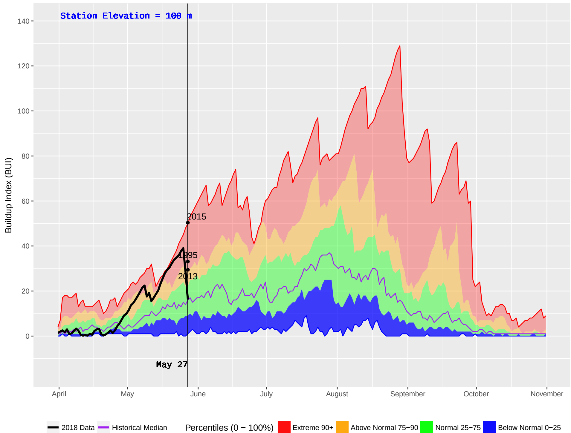
HONNA (93) : Historical (1986–2016) and Current (2018) Noon Buildup Index (BUI)
