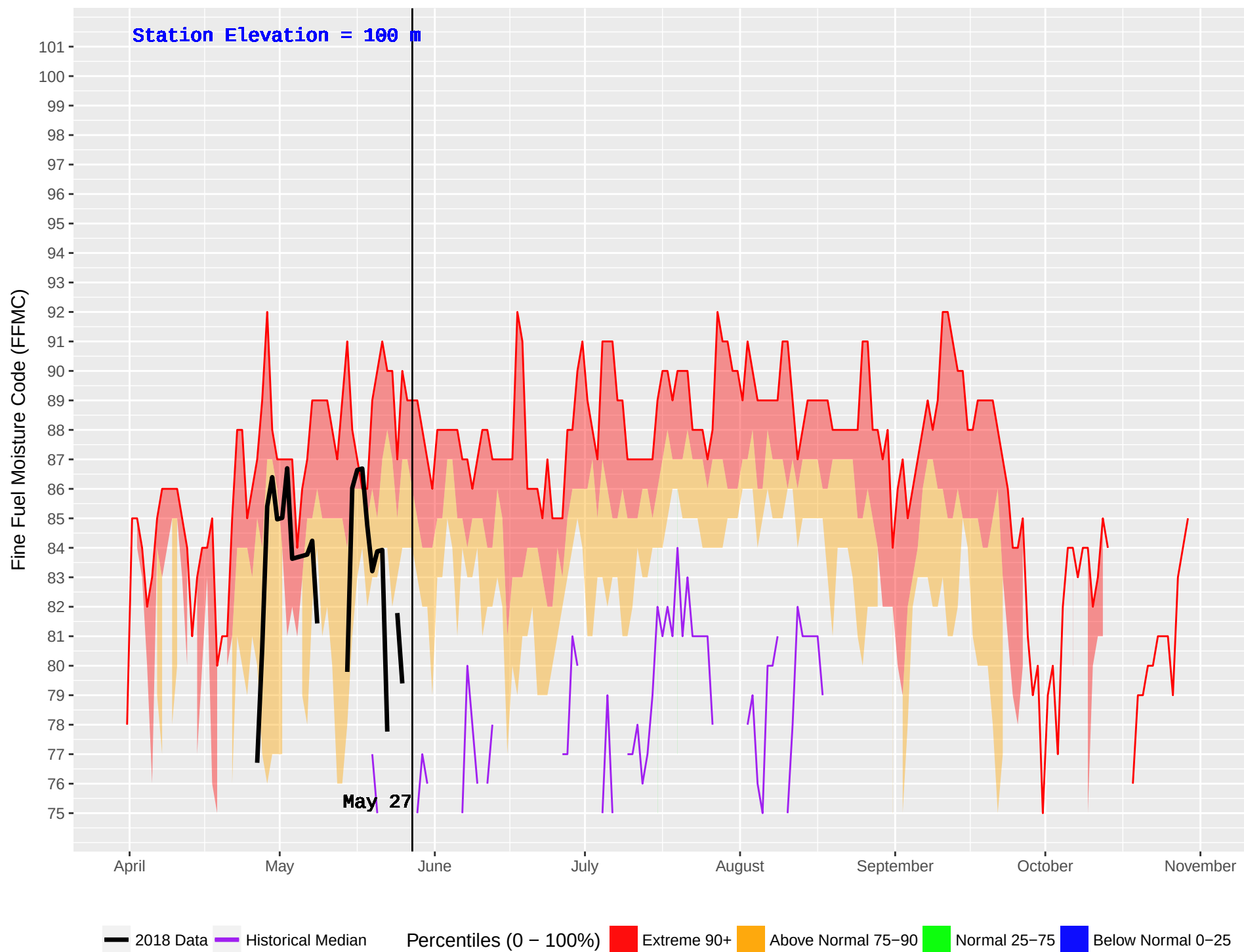
HONNA (93) : Historical (1986–2016) and Current (2018) Noon Fine Fuel Moisture Code (FFMC)
