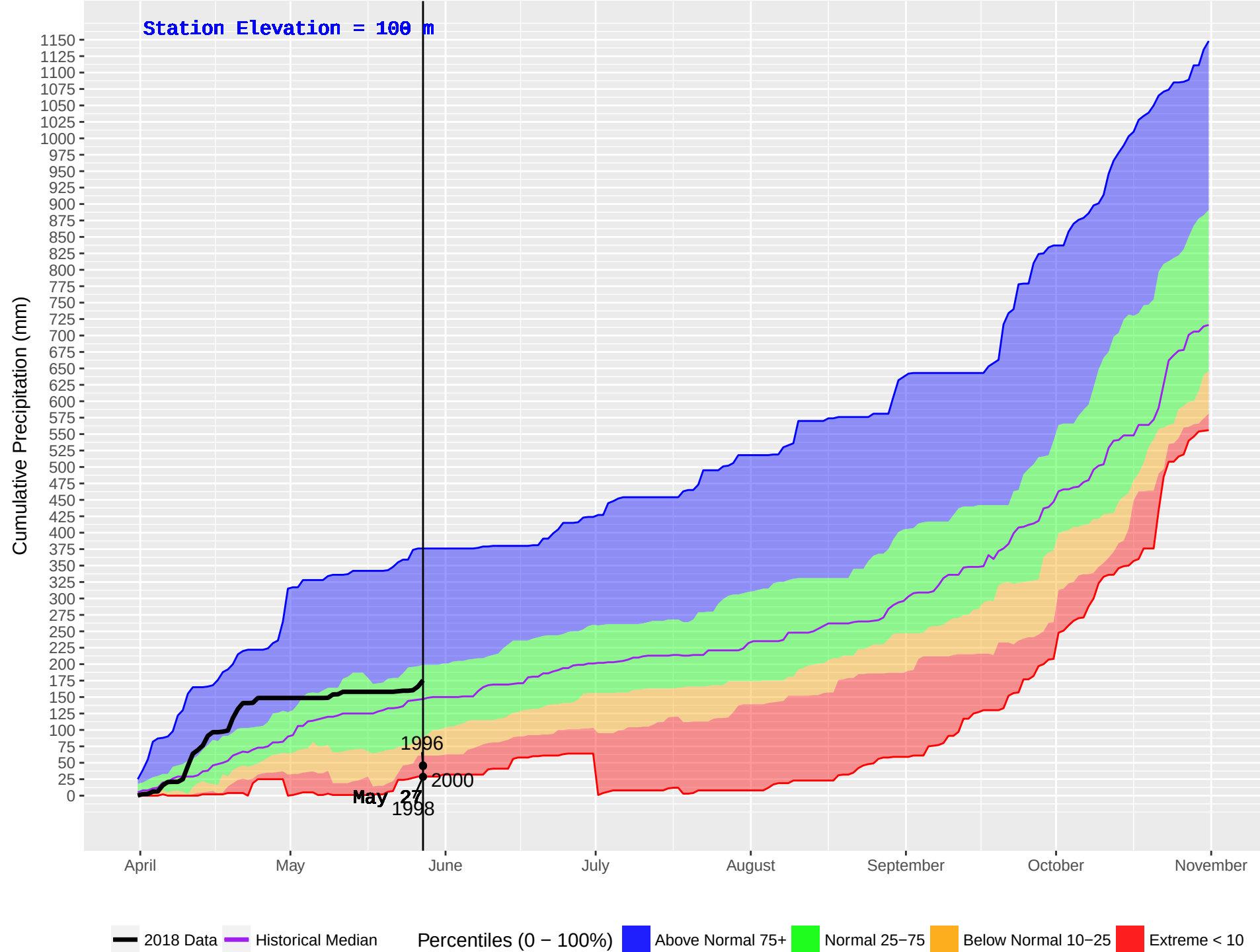
HONNA (93) : Historical (1986–2016) and Current (2018) Noon Cumulative Precipitation
