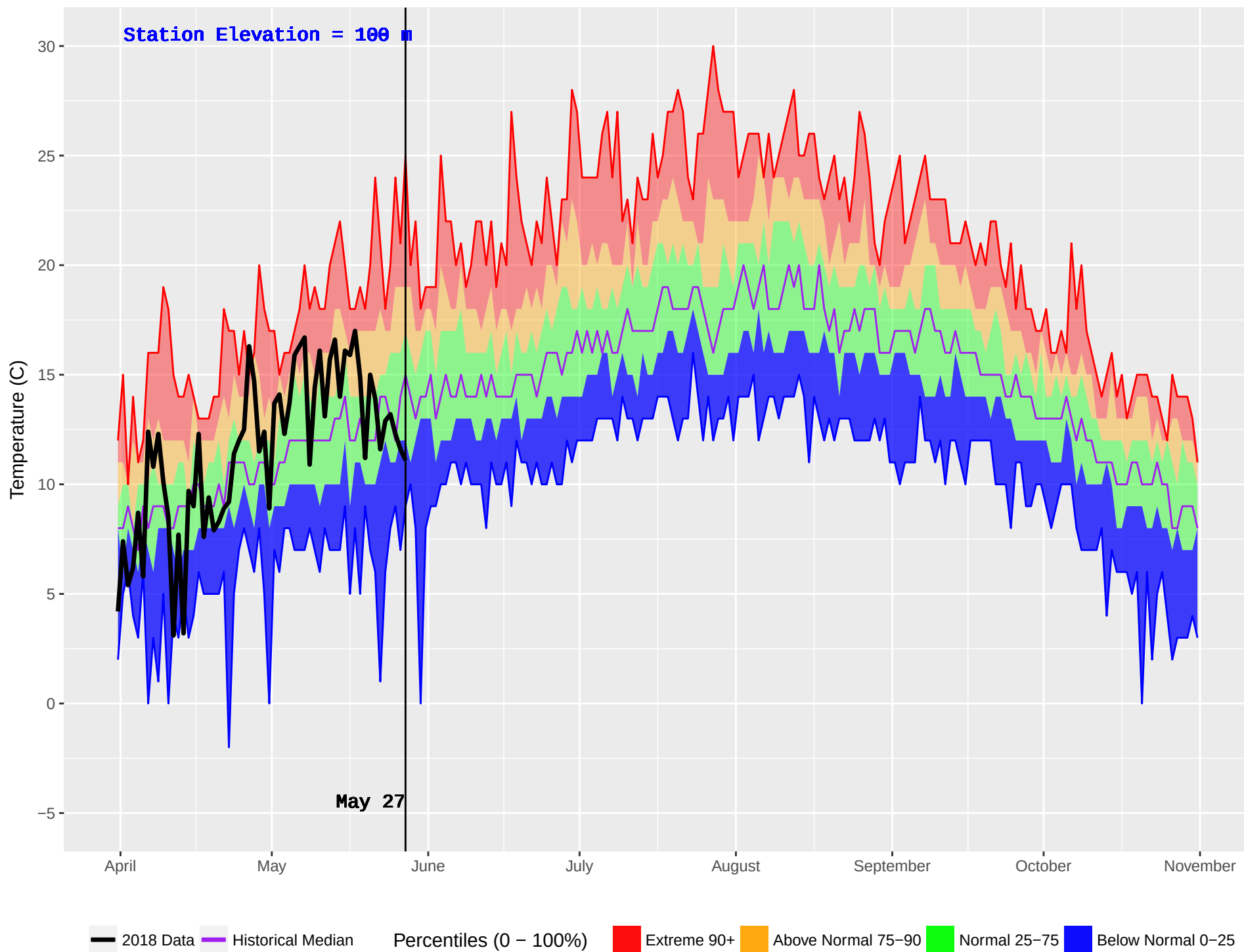
HONNA (93) : Historical (1986–2016) and Current (2018) Noon Temperature
