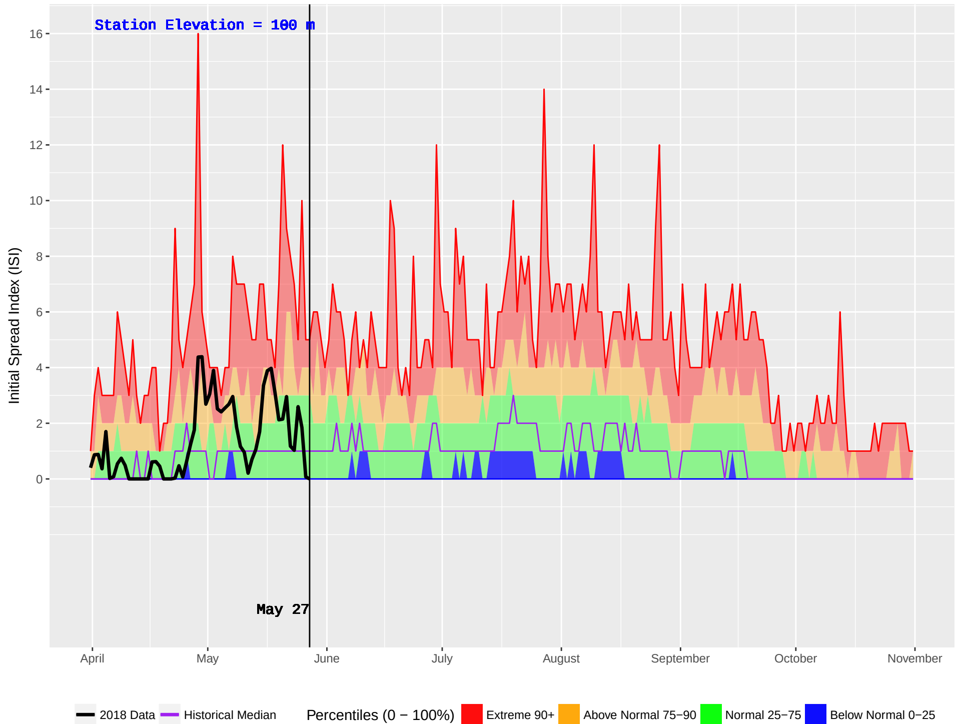
HONNA (93) : Historical (1986–2016) and Current (2018) Noon Initial Spread Index (ISI)
