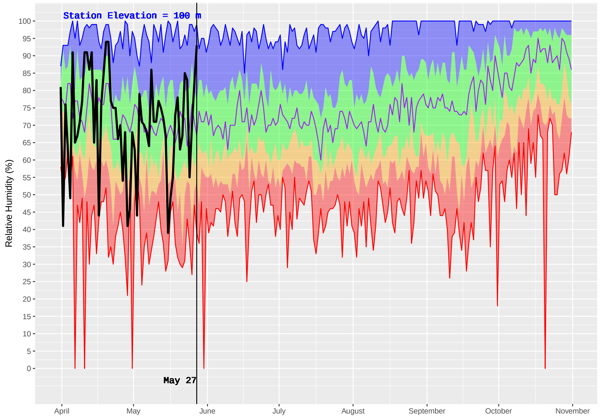
HONNA (93) : Historical (1986–2016) and Current (2018) Noon Relative Humidity
